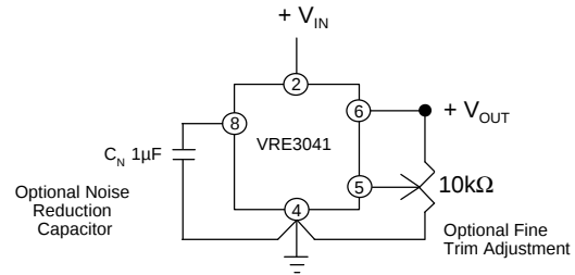
Figure 3 External Connections
