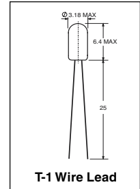
T-1/4 Bi-Pin
