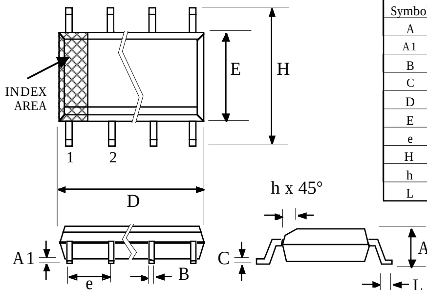
16 pin SOIC narrow
