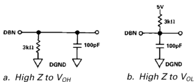
FIGURE 1. LOAD CIRCUITS FOR ACCESS TIME ( t_6 )
