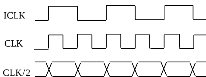
x2 Mode (S1, S0 = 1, 1) CLK Feedback
