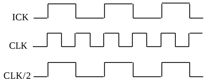
x2 Mode (S1, S0 = 1, 0) CLK/2 Feedback
