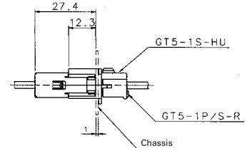
Assembly Diagram (1:1)
