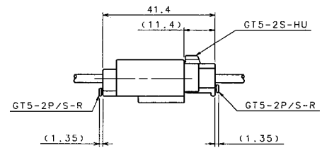
◆ Diagram of Mated Connector in Use
