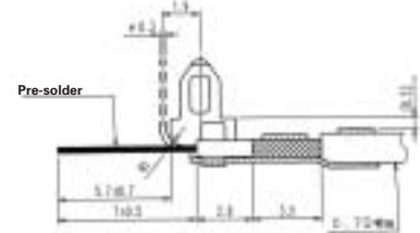
Completed Termination Cross Section
