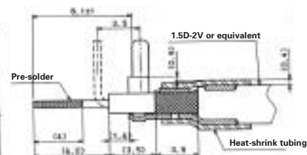
◆ Completed Termination cross section
