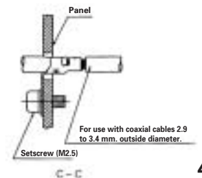
Attachment Diagram
