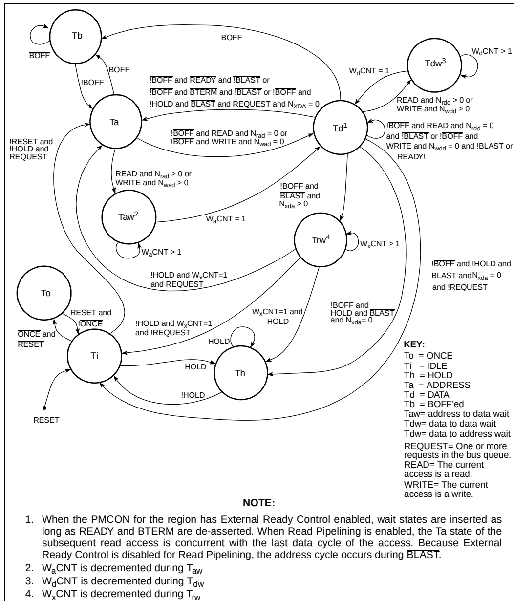
Figure 59. Bus States
