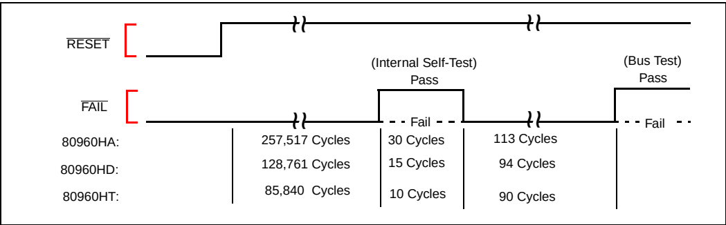
Figure 53. \overline{\text{FAIL}} Functional Timing
