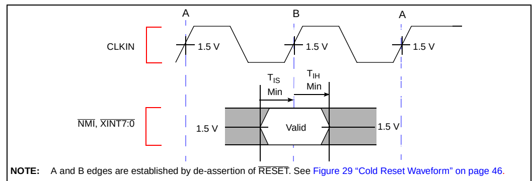
Figure 14. \overline{NMI} , \overline{XINT7:0} Input Setup and Hold Waveform
