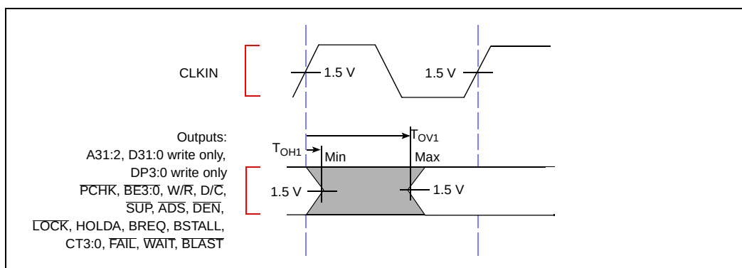
Figure 11. Output Delay Waveform
