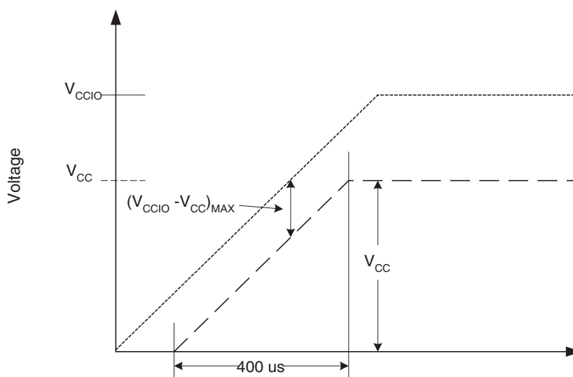
Figure 30: Power-up Sequencing
