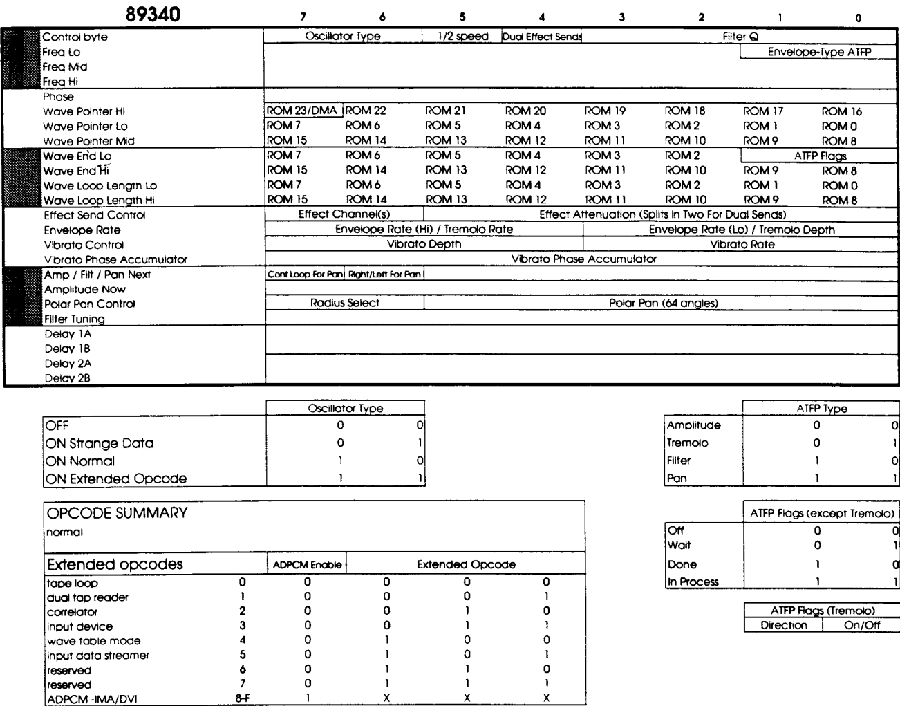
Figure 10. General-Purpose Oscillator Address Map
