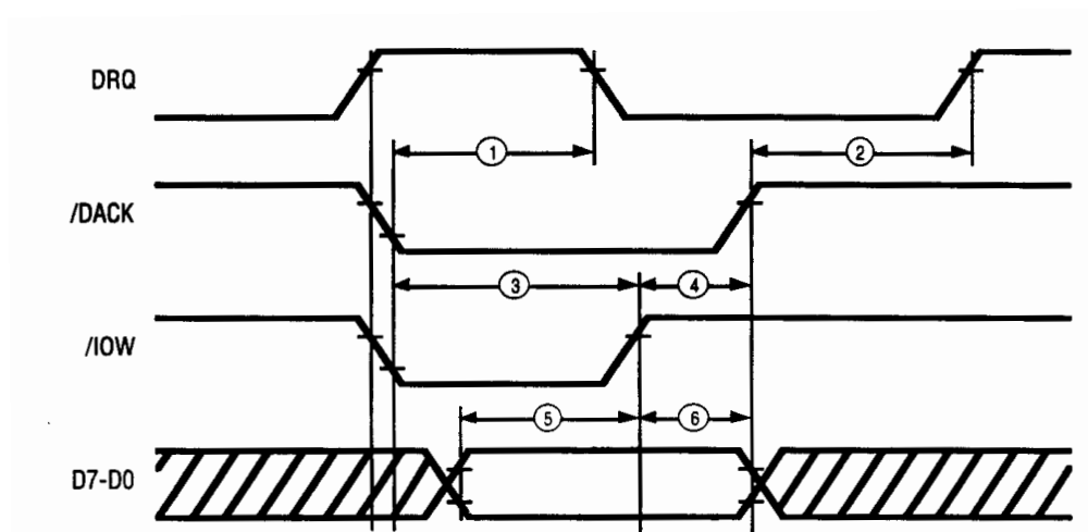
Figure 3. DMA Write Timing Diagram
