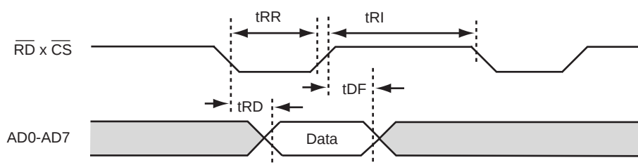
FIGURE 3(a) MICROPROCESSOR READ CYCLE IN INTEL BUS MODE
