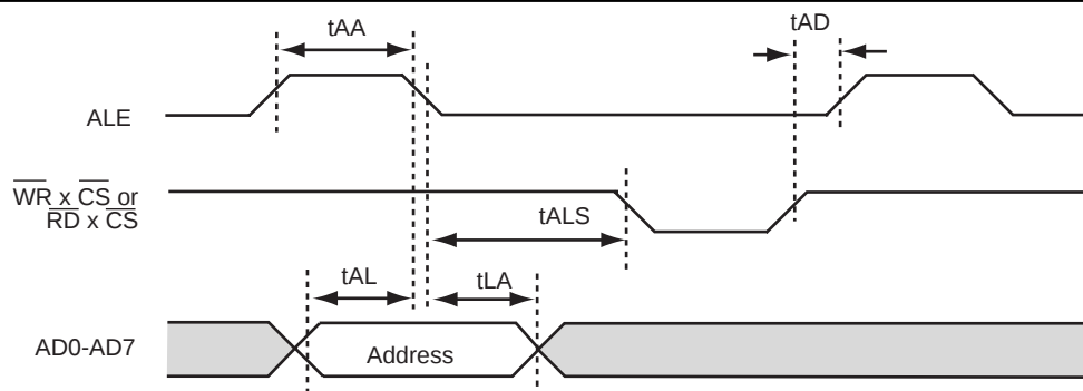
FIGURE 3(b) MICROPROCESSOR WRITE CYCLE IN INTEL BUS MODE
