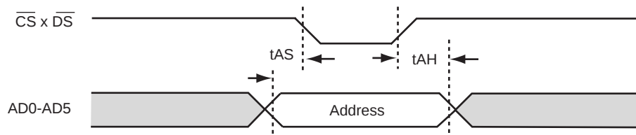
FIGURE 4(c) NON-MULTIPLEXED ADDRESS TIMING IN MOTOROLA BUS MODE
