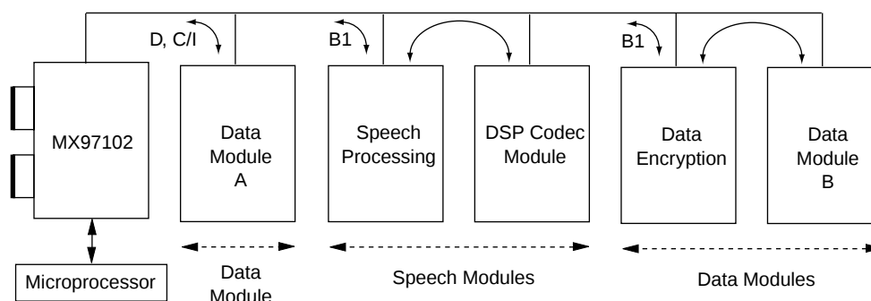
FIGURE 6: EXAMPLES OF GCI CONNECTION
