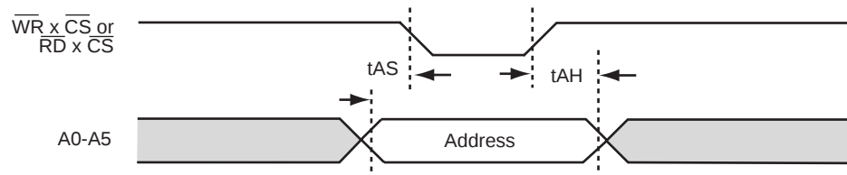
FIGURE 3(d) NON-MULTIPLEXED ADDRESS TIMING IN INTEL BUS MODE
