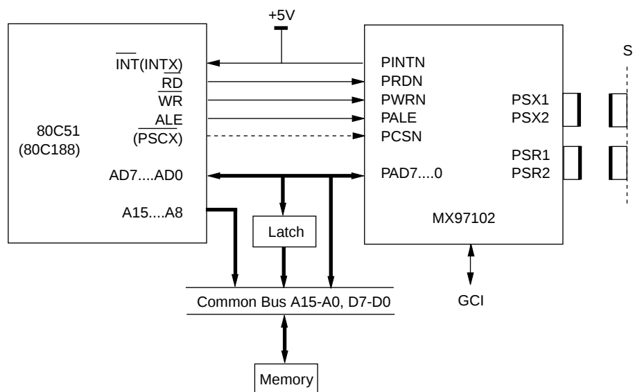
FIGURE 7: CONNECTING THE MX97102 TO INTEL MICROCONTROLLER
