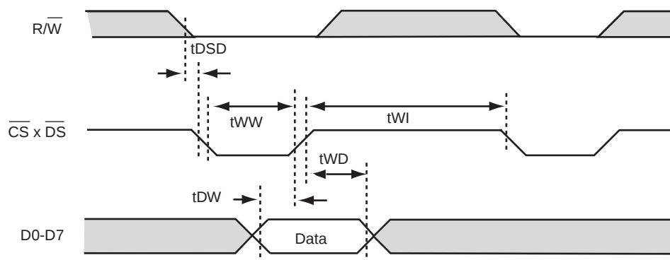
FIGURE 4(b) MICROPROCESSOR WRITE TIMING IN MOTOROLA BUS MODE
