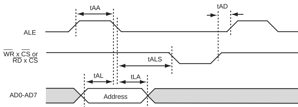
FIGURE 3(c) MULTIPLEXED ADDRESS TIMING IN INTEL BUS MODE
