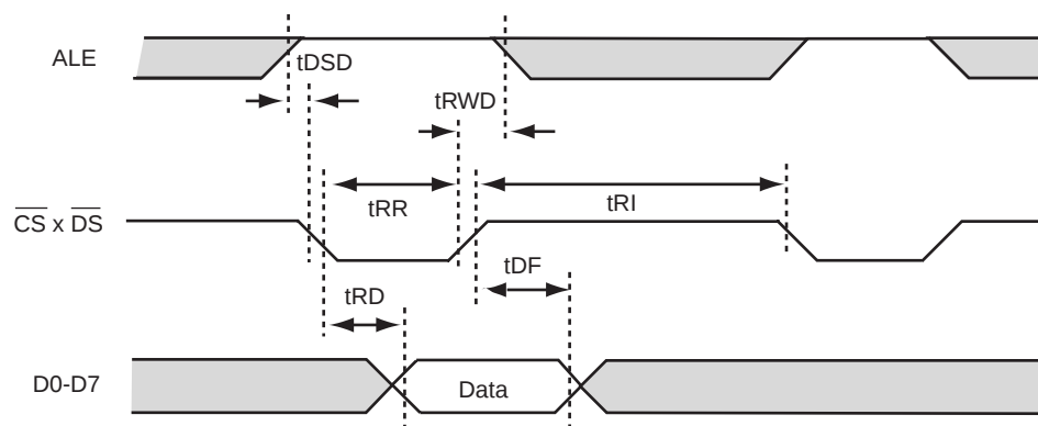
FIGURE 4(a) MICROPROCESSOR READ TIMING IN MOTOROLA BUS MODE
