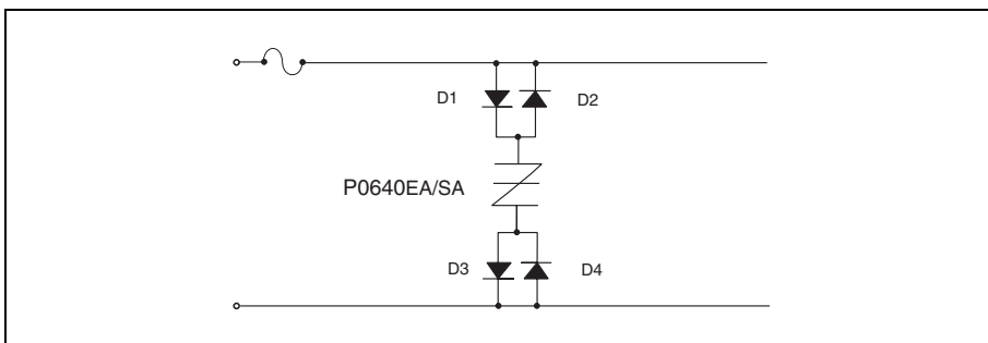
Figure 3.45 100 Base-T Protection
