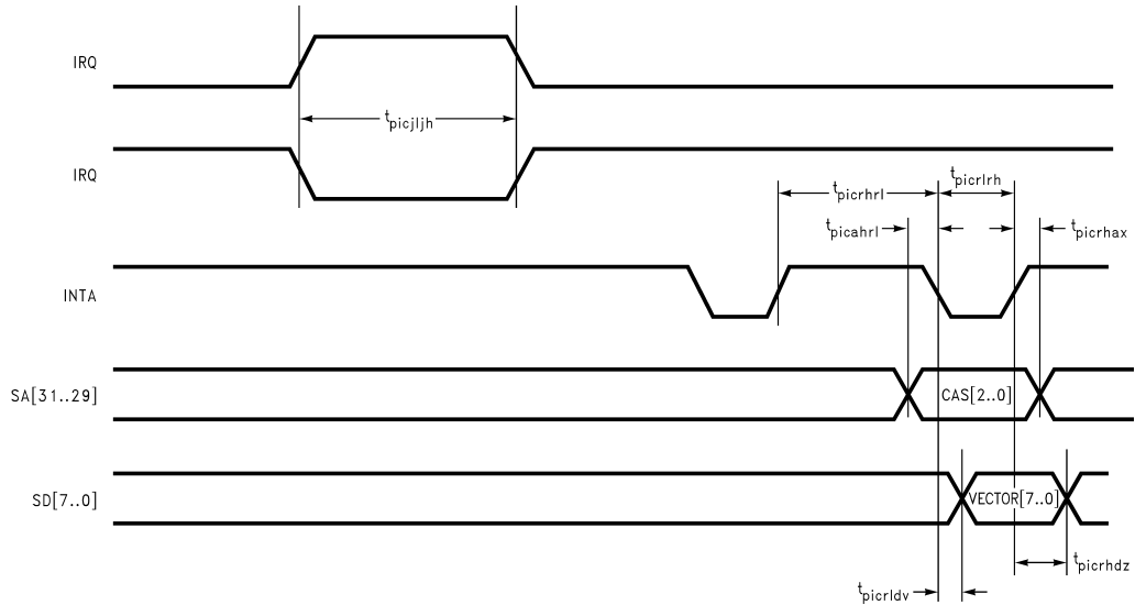
FIGURE 12. PIC Timing Diagram
