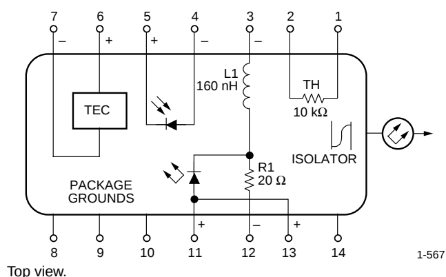
Figure 1. Circuit Schematic
