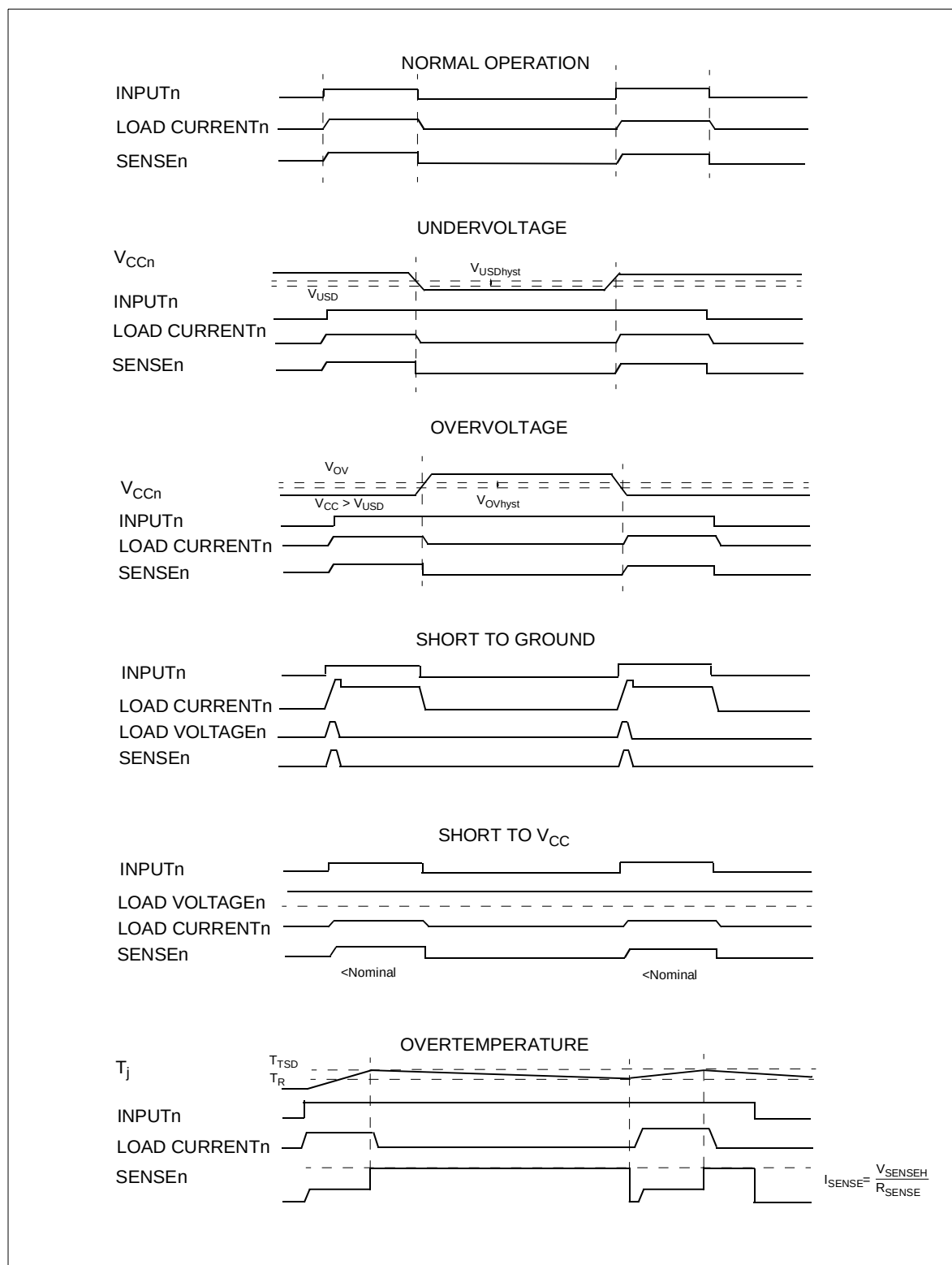
Figure 3: Waveforms
