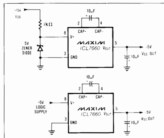
Figure 15. Generating -5V for V_{SS}
