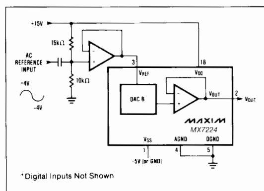
Figure 14. AC Reference Input Circuit
