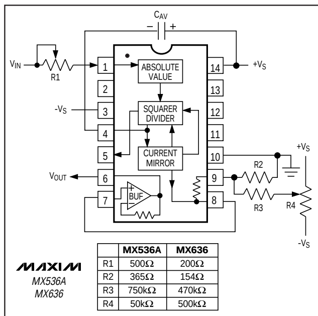
Figure 4. Optional External Gain and Output Offset Trims
