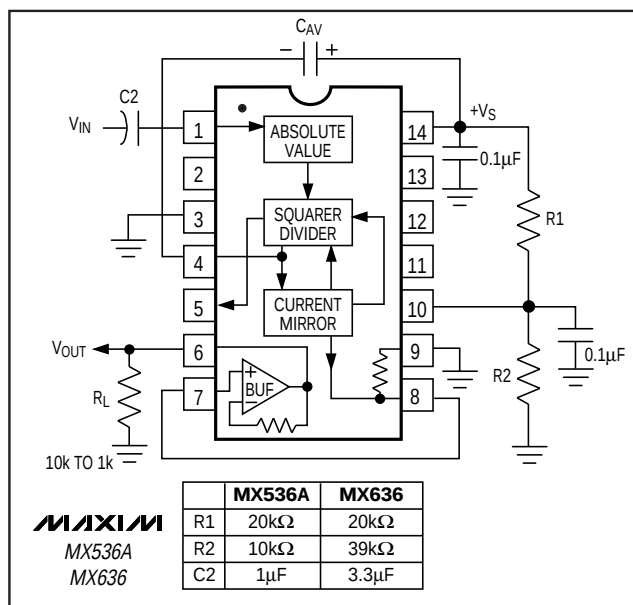
Figure 5. Single-Supply Operation
