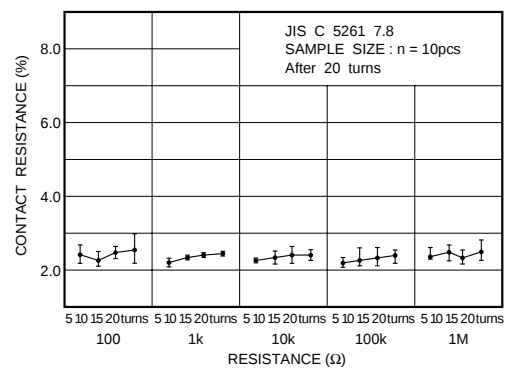
Fig.6-2 Endurance (wiper)
