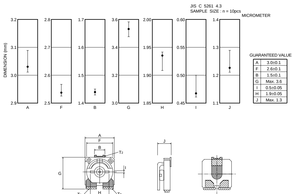
Fig.2 Dimensions
