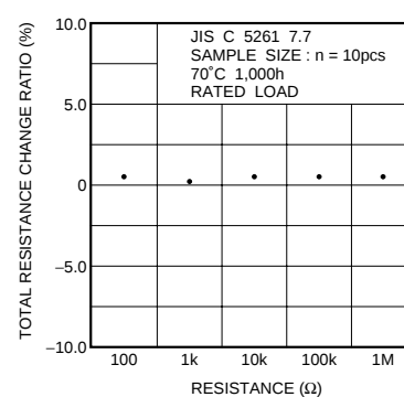
Fig.13-1 Endurance (rated load)
