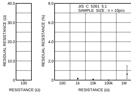
Fig.4 Residual resistance
