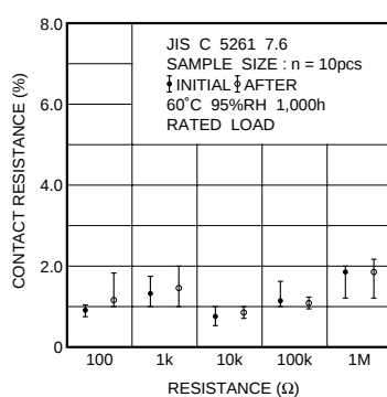
Fig.12 Endurance (Under load in damp environment)
