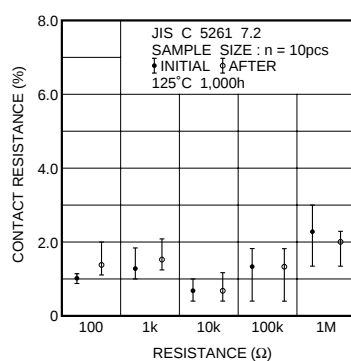
Fig.9 Resistance to dry heat
