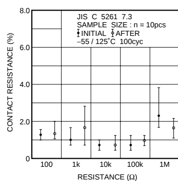
Fig.10-2 Temperature cycling
