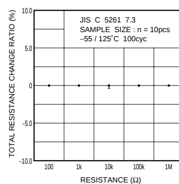
Fig.10-1 Temperature cycling
