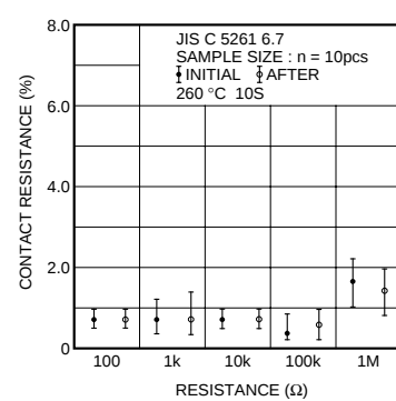
Fig.8 Resistance to soldering heat
