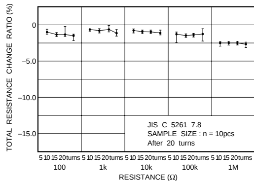
Fig.6-1 Endurance (wiper)
