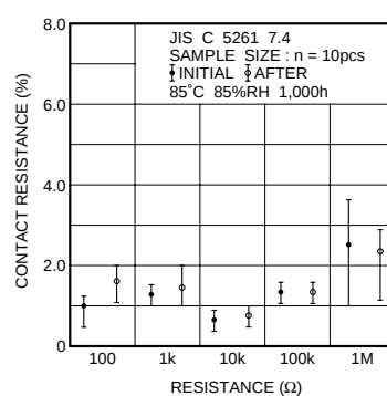
Fig.11 Resistance to humidity (steady state)
