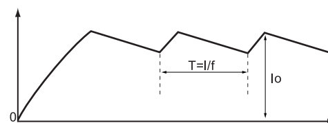
Fig.1 Constant current wave form (Motor current / phase)
