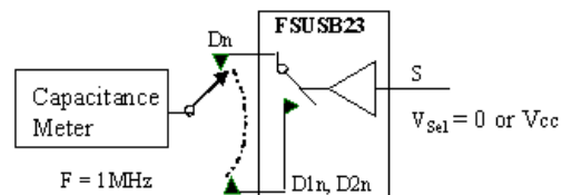
FIGURE 11. Channel OFF Capacitance
