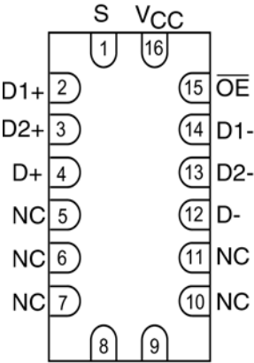
Pad Assignments for DQFN
