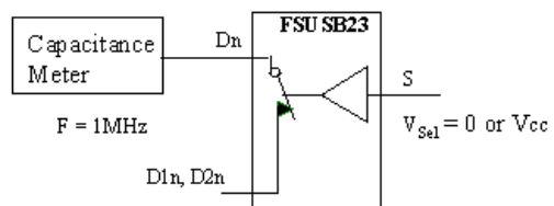
FIGURE 10. Channel ON Capacitance
