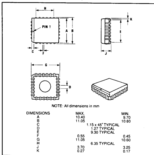
Fig.11 FX439LS Package
