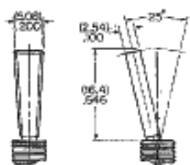
Q4 .840" Cone (available on 1 & 2-pole only)
