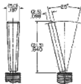
E4 .840" Flatted (available on 1 & 2-pole only)
