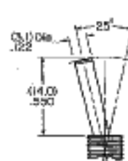
D .840" Color Capped Cone (available on 1 & 2-pole only)
