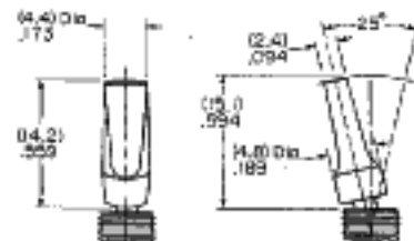
K2 .559" Paddle
