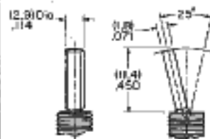
C .571" Color Tipped Cone (available on 1 & 2-pole only)
