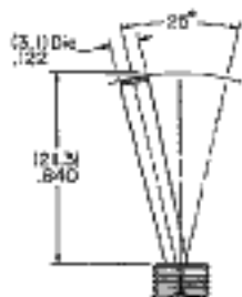
Q4 .840" Cone (available on 1 & 2-pole only)
