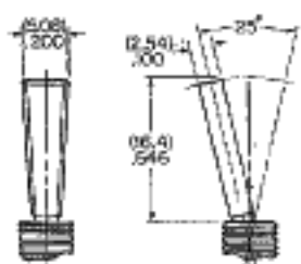
Q4 .840" Cone (available on 1 & 2-pole only)
