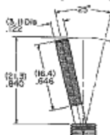
D .840" Color Capped Cone (available on 1 & 2-pole only)
