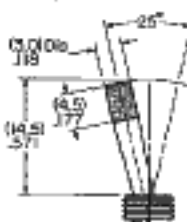
C .571" Color Tipped Cone (available on 1 & 2-pole only)
