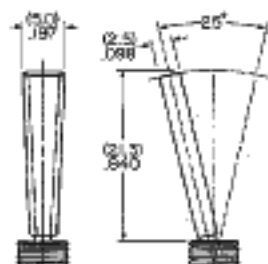
E4 .840" Flatted (available on 1 & 2-pole only)
