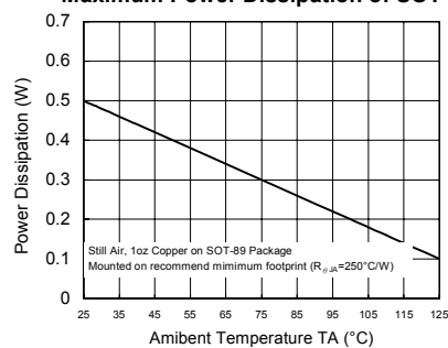
Maximum Power Dissipation of SOT-89
