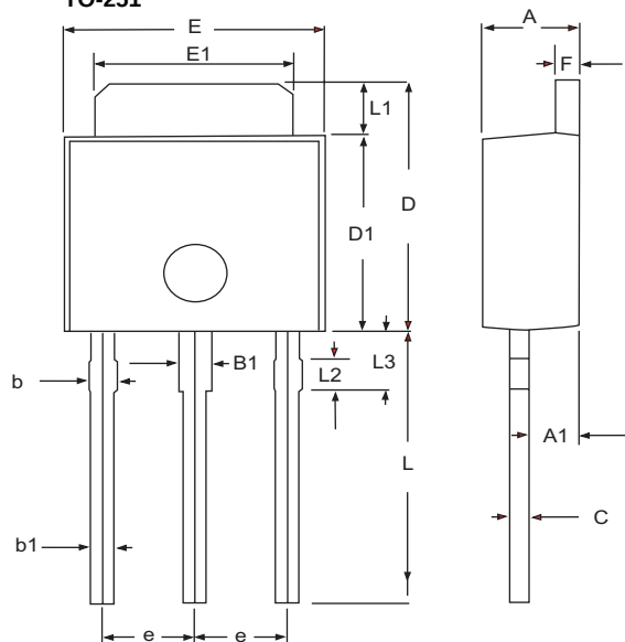
TO-251
