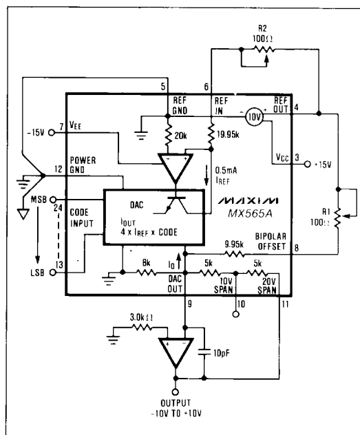
Figure 4(c). MX565A \pm 10V Bipolar Voltage Output
