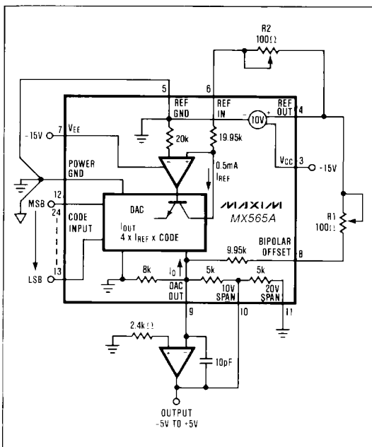
Figure 4(b). MX565A \pm 5V Bipolar Voltage Output
