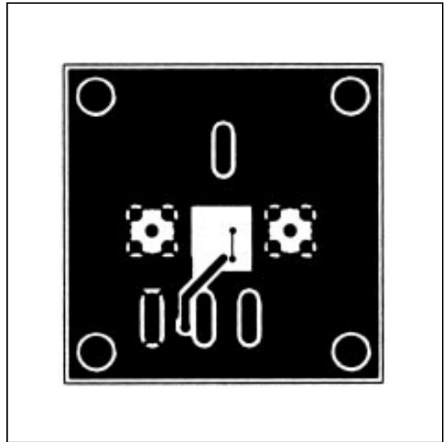
Figure 7c. Maxim SOT23 High-Speed Evaluation Board PCB Board Layout—Back Side
