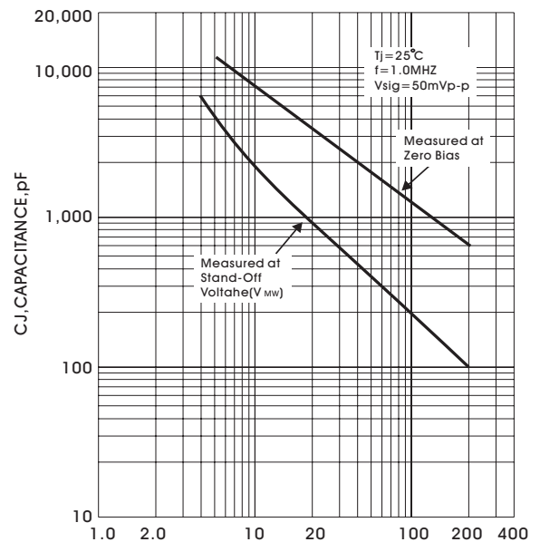
FIGURE 4 TYPICAL CAPACITANCE VS STAND-OFF VOLTAGE
