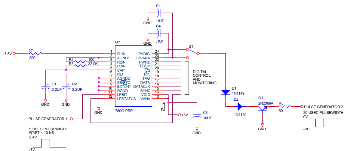
FIGURE 8. 7809LP LPT™ TEST CIRCUIT
