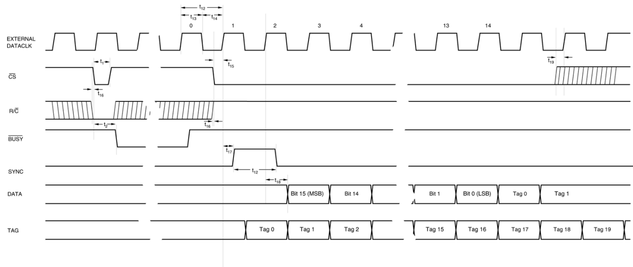
FIGURE 3. CONVERSION AND READ TIMING WITH EXTERNAL CLOCK (EXT/ \overline{INT} TIED HIGH). READ AFTER CONVERSION
