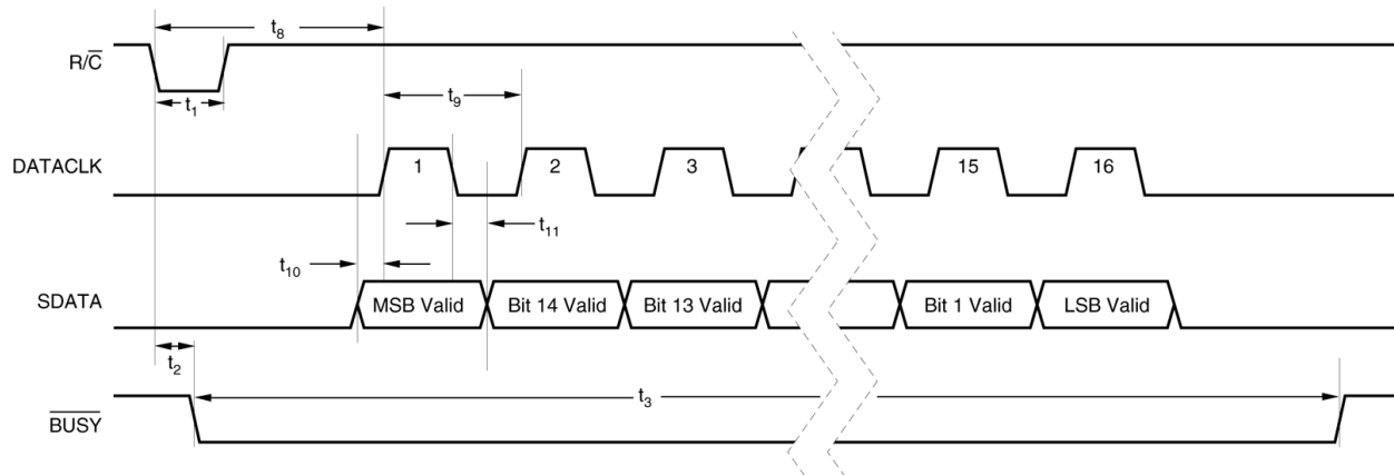
FIGURE 2. SERIAL DATA TIMING USING INTERNAL CLOCK ( \overline{CS} , EXT/ \overline{INT} AND TAG TIED LOW)
