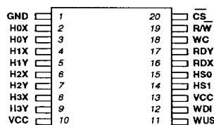
4-Channel 20-lead SOIC, SSOP, VSOP
