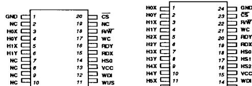
2-Channel 20-lead SSOP 6-Channel 24-lead SSOP
