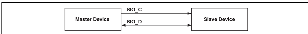
Figure 1-2 2-Wire SCCB Functional Block Diagram
