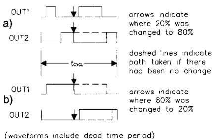
Fig. 7 Effect of Changing the Duty Cycle during a PWM Cycle
