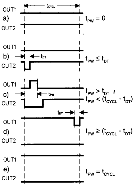
Fig. 6 Effect of Nonzero Dead-time on PWM Waveform
