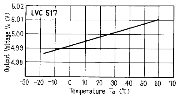
LVC517 温度特性/Temperature Charac.
