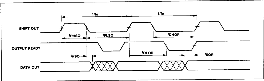
Fig.9 Switching waveforms - Data Out timing
