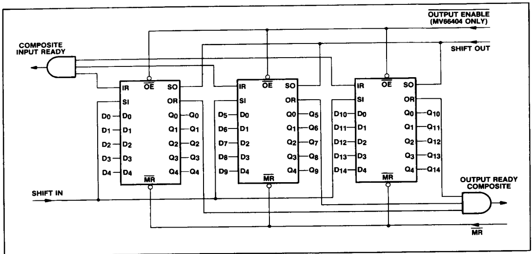
Fig.10 64 x 15 application (MV65402/MV65404)
