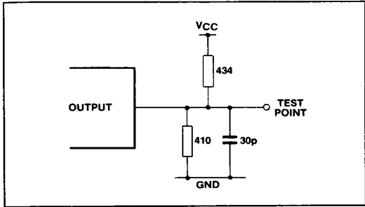
Fig.3 Test circuit
