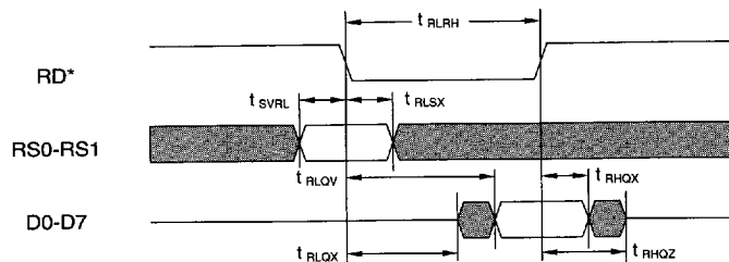
Basic Read Cycle Timing
