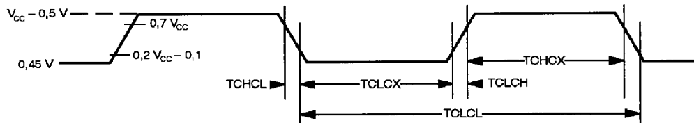
Figure 10. Clock Signal Waveform for ICC Tests in Active and Idle Modes. TCLCH = TCHCL = 5 ns.
