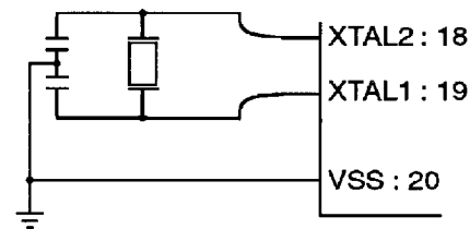
Figure 5. Crystal Oscillator.
