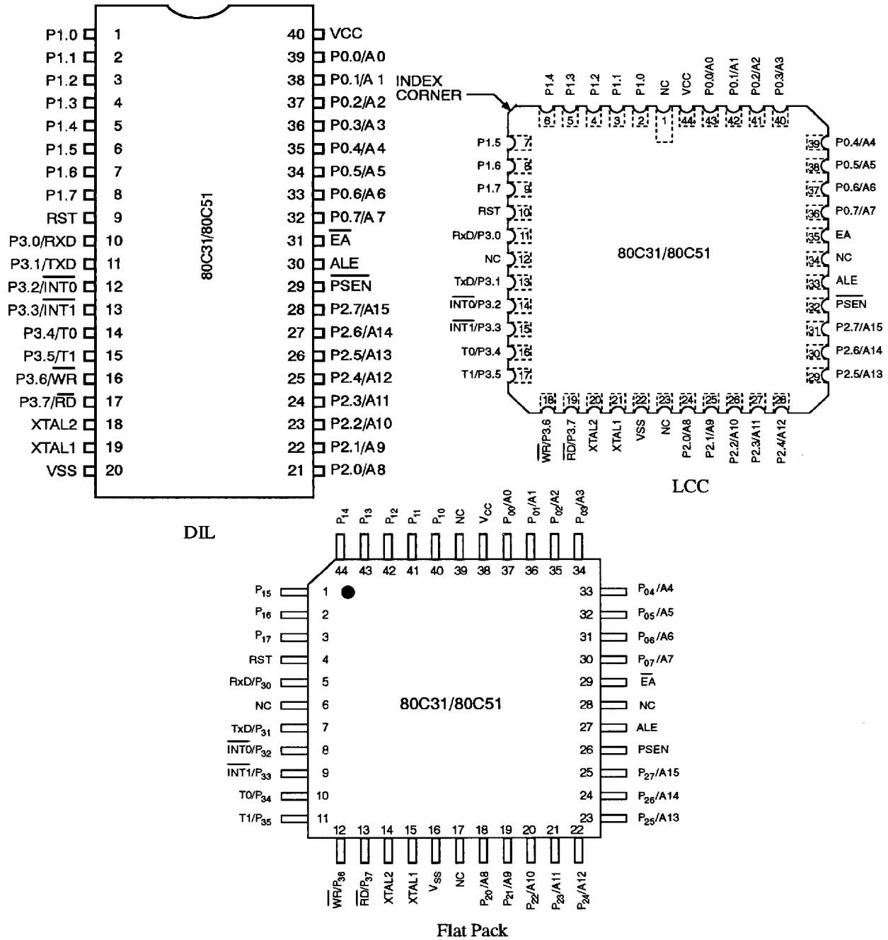
Figure 2. Pin Configuration
