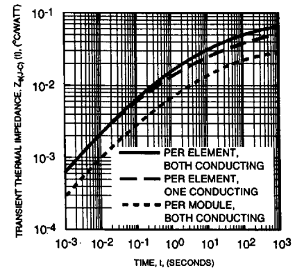
TRANSIENT THERMAL IMPEDANCE CHARACTERISTICS (JUNCTION-TO-CASE) Z JA
