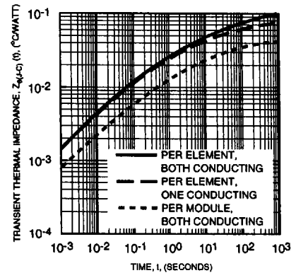
TRANSIENT THERMAL IMPEDANCE CHARACTERISTICS (JUNCTION-TO-CASE) Z JA
