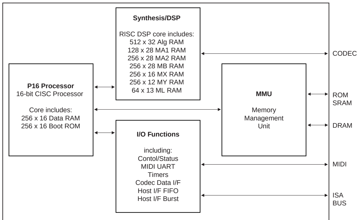
Figure 4. IC Architecture
