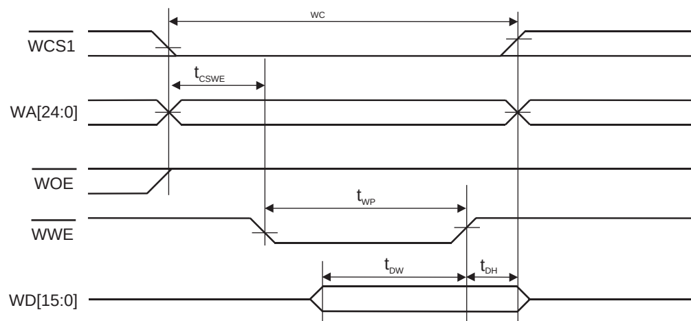
Figure 12. 16-bit SRAM Write Cycle
