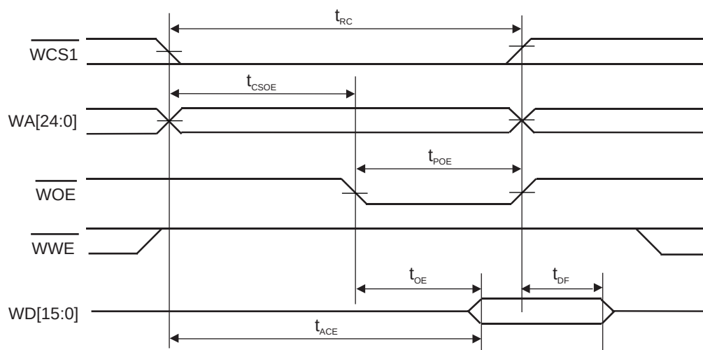
Figure 11. 16-bit SRAM Read Cycle
