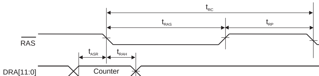
Figure 9. External DRAM Refresh Cycle ( \overline{\text{RAS}} Only)
