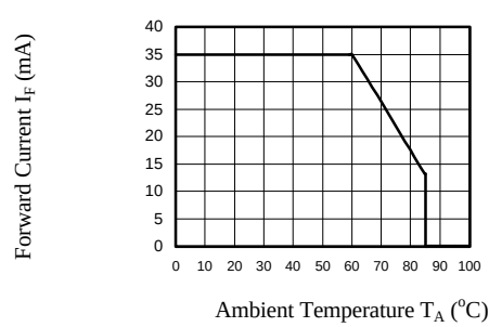
FIG.3 FORWARD CURRENT VS. AMBIENT TEMPERATURE
