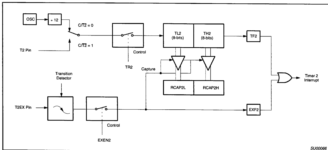
Figure 2. Timer 2 in Capture Mode
