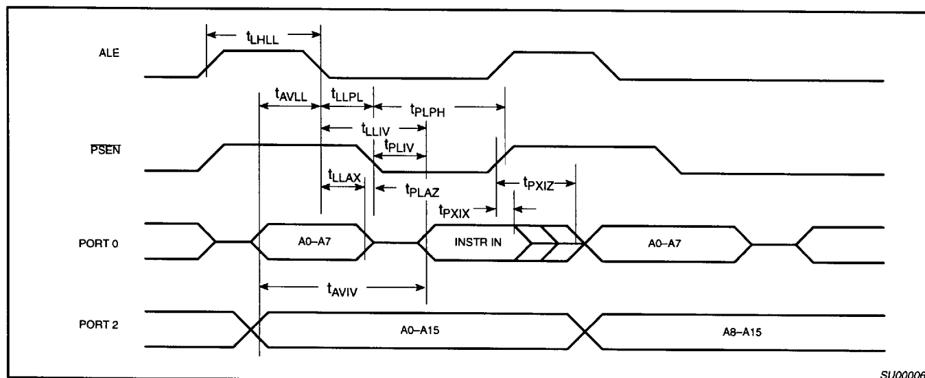
Figure 5. External Program Memory Read Cycle
