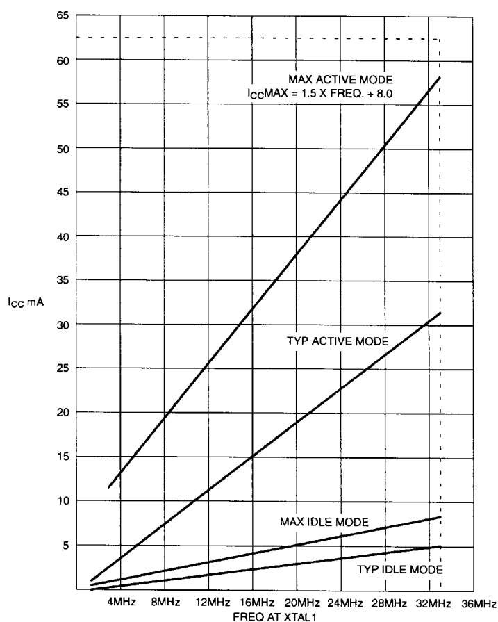
Figure 12. I_{CC} vs. FREQ
