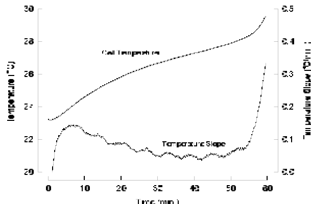
Figure 7: Cell temperature and temperature slope
