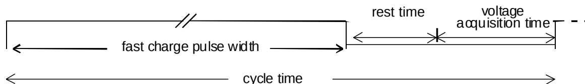
Figure 4: Charge cycle showing fast charge current pulses
