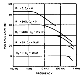
Figure 12. Op Amp Frequency Response
