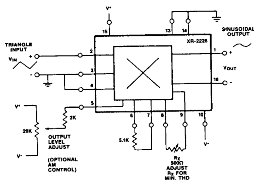
Figure 19. Triangle-to-Sinewave Converter
