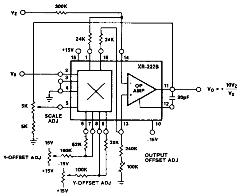
Figure 15. Dividing Circuit
