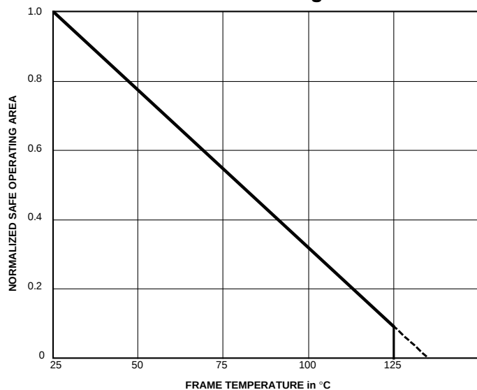
S.O.A. Derating
