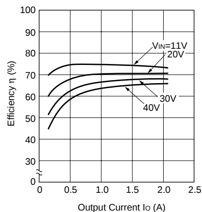
Efficiency Characteristics
