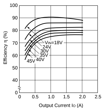
Efficiency Characteristics
