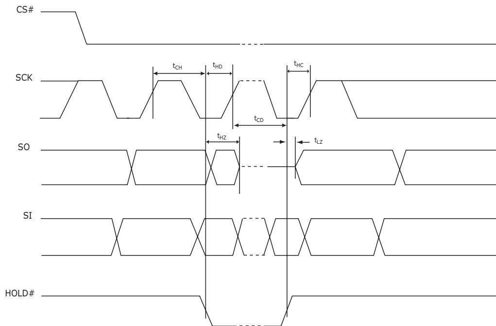
Figure 21. HOLD# Timing
