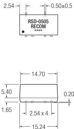
Dual SMD Package
