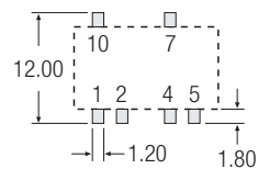
Recommended Footprint Details
