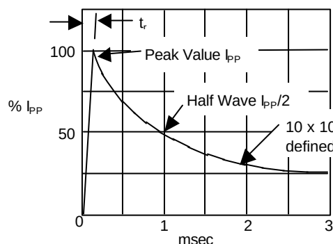
Figure 1 - Pulse Waveform
