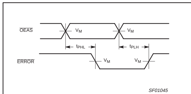
Waveform 3. Propagation Delay, Output Enable to ERROR
